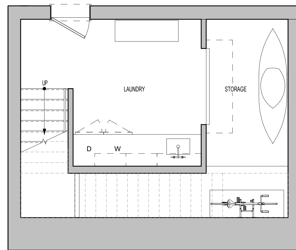
1 BASEMENT PLAN 1/4" = 1'-0"
