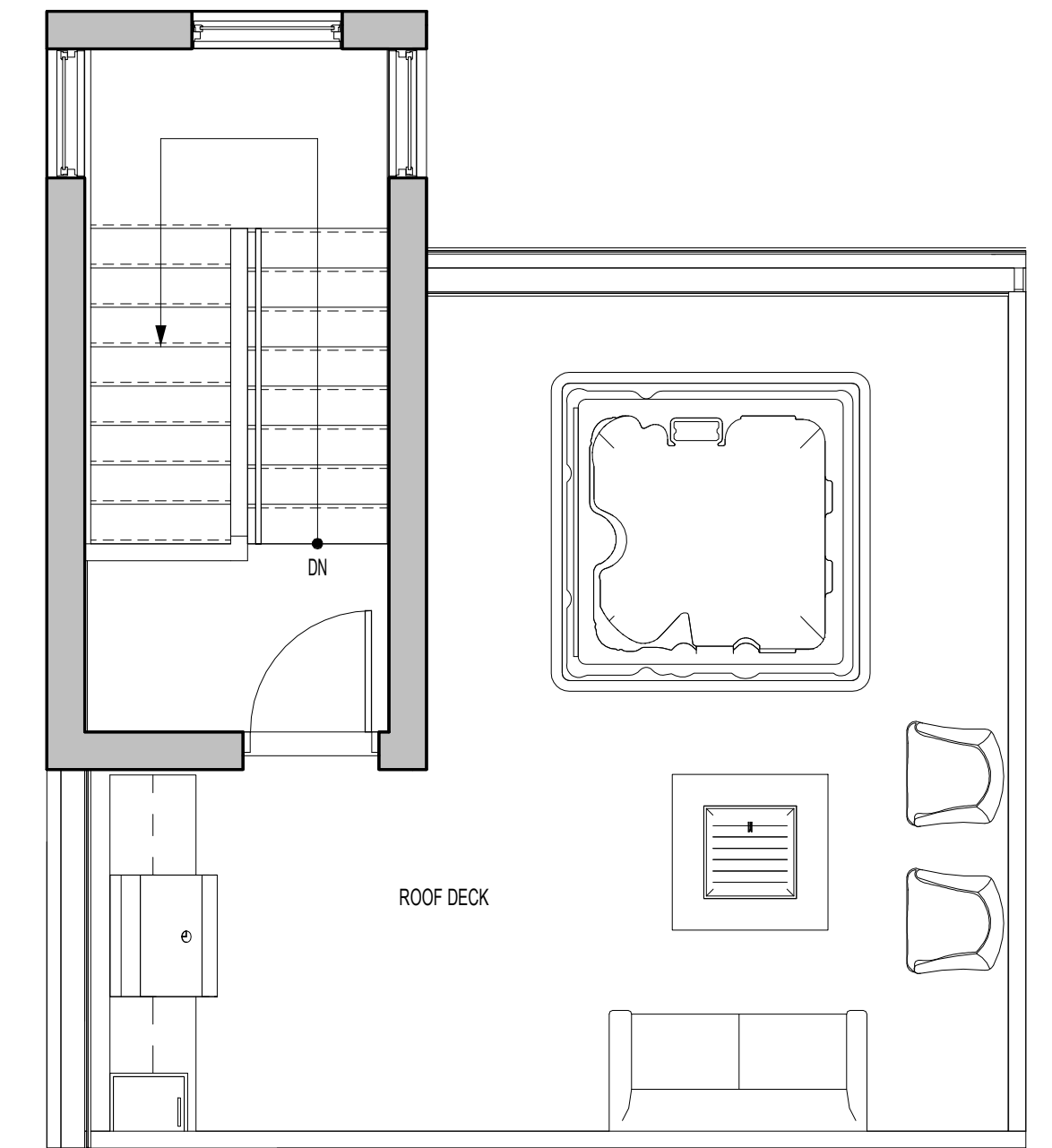
5 ROOF PLAN 1/4" = 1'-0"
