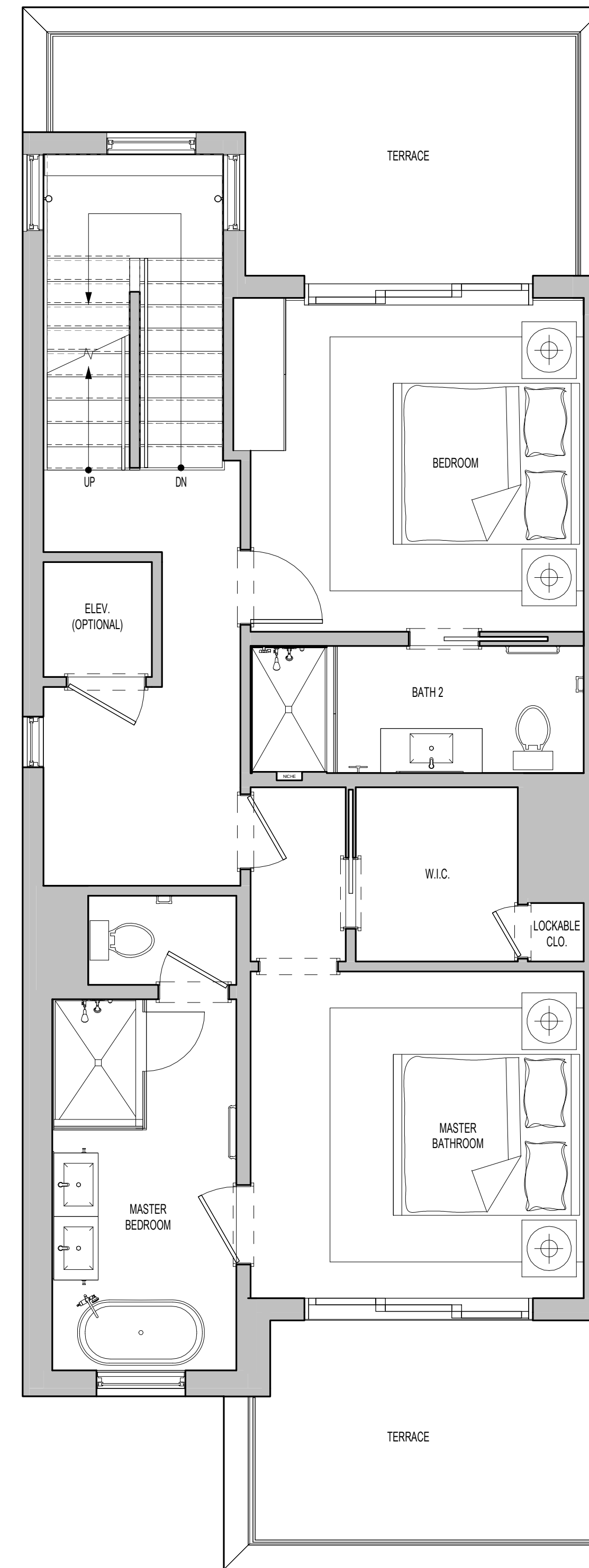
4 THIRD FLOOR PLAN 1/4" = 1'-0"
